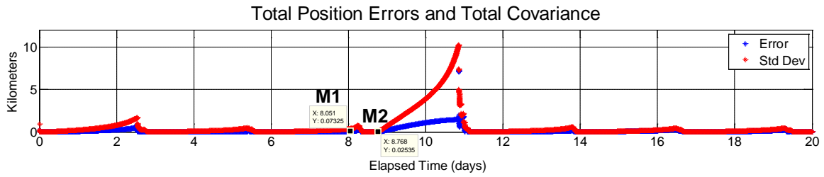
Figure 17. Baseline RSS Position Error and Covariance.
