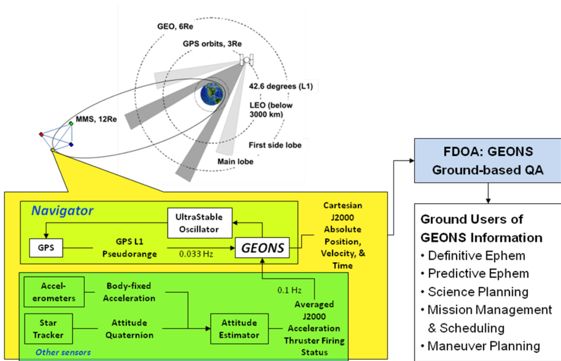
Figure 1. Navigation Concept and Onboard Configuration.
